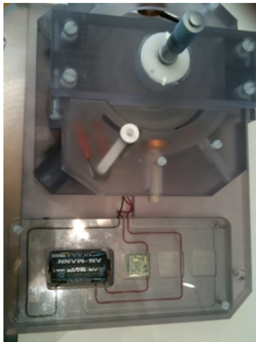
The electromagnetic Orbo Device on display - Photo Courtesy of ESA
