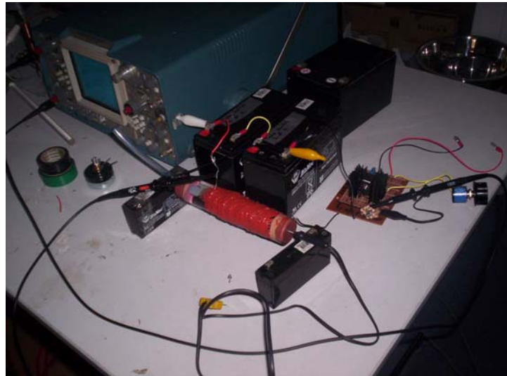
Panacea's Rosemary Ainslie heating circuit
